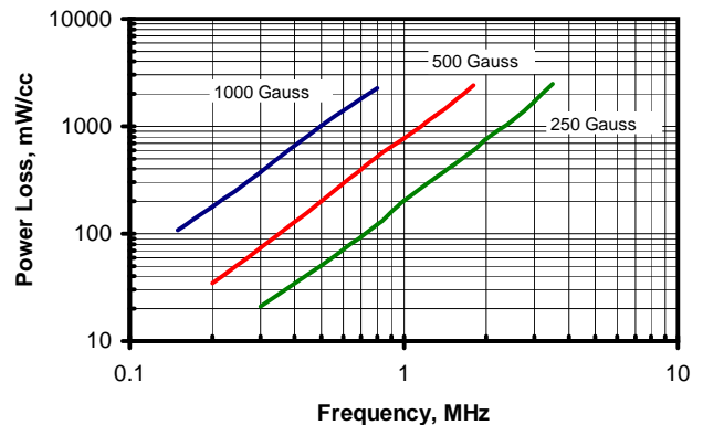
Power Loss vs. Frequency
