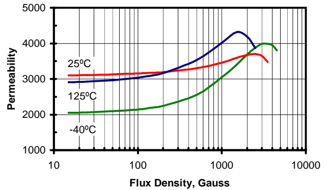
Permeability vs. Flux Density
