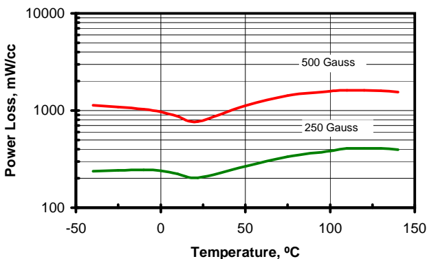
Power Loss vs. Temperature at 1 MHz
