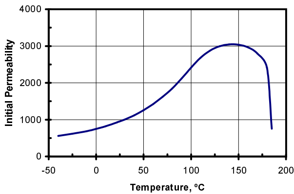
Initial Permeability vs. Temperature at 500 KHz
