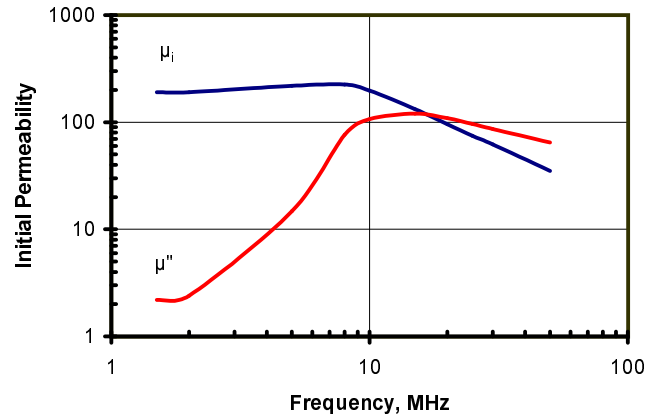
Complex Permeability vs. Frequency
