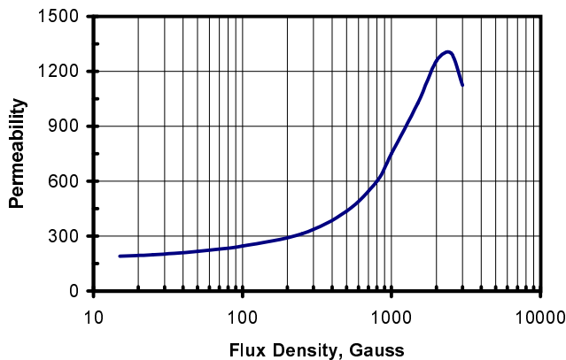
Permeability vs. Flux Density
